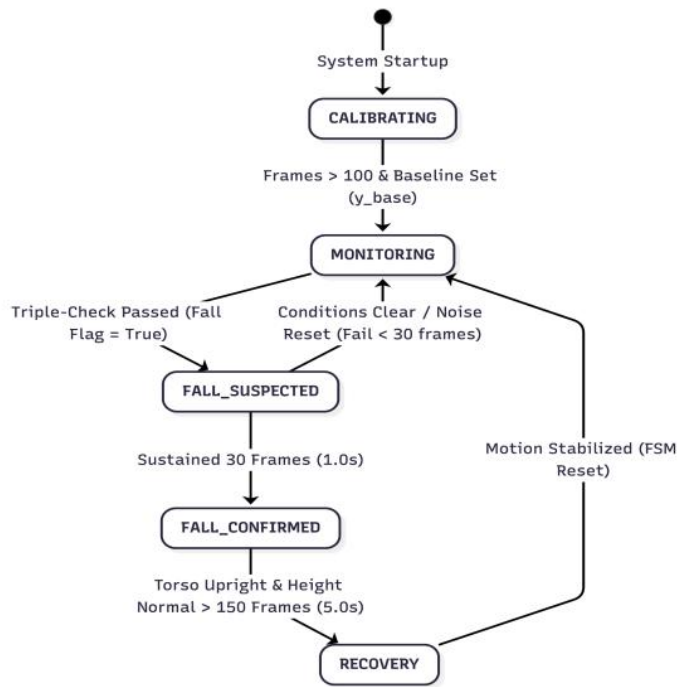
Figure 3: State-machine architecture.
