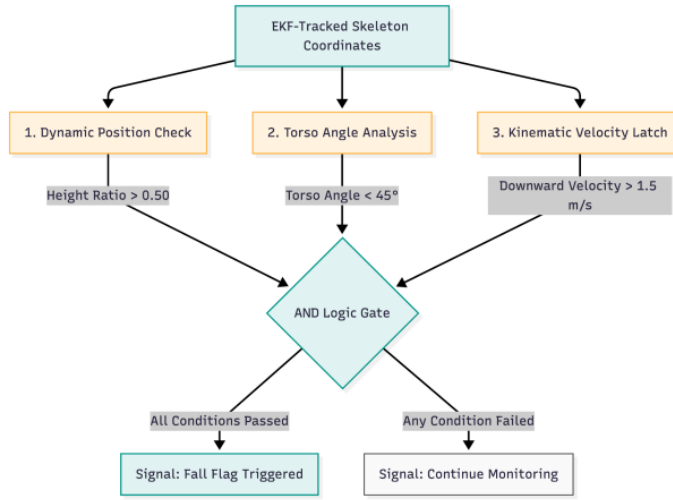
Figure 2: DAIO uses a parallel multi-metric evaluation architecture.
