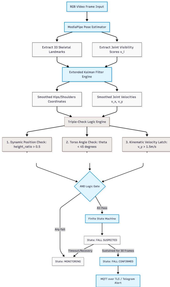
Figure 1: System architecture.
